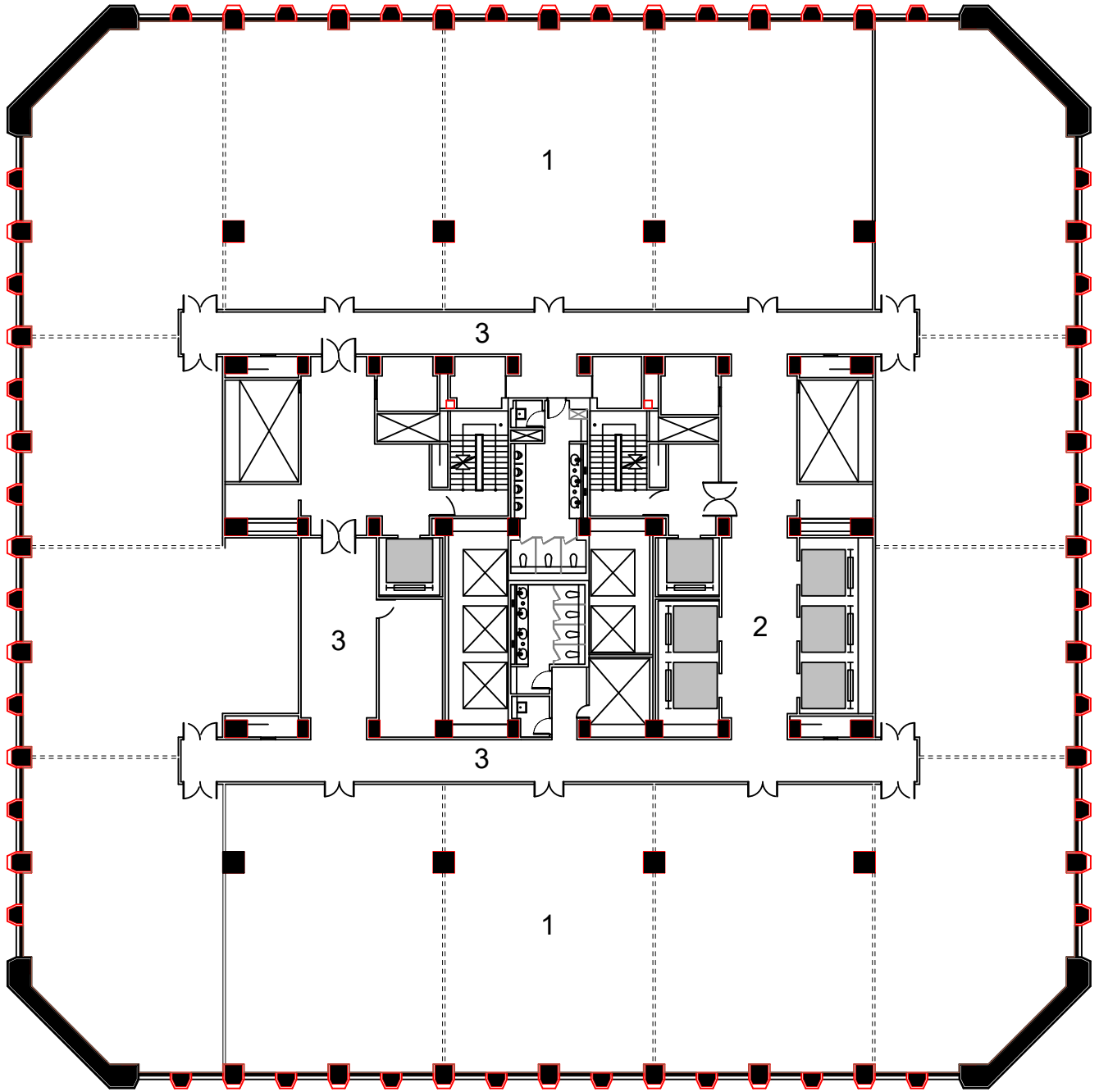
Typical floor plan (14~23)
